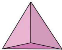
triangular-based pyramid
