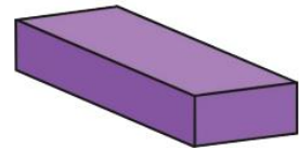
cuboid
